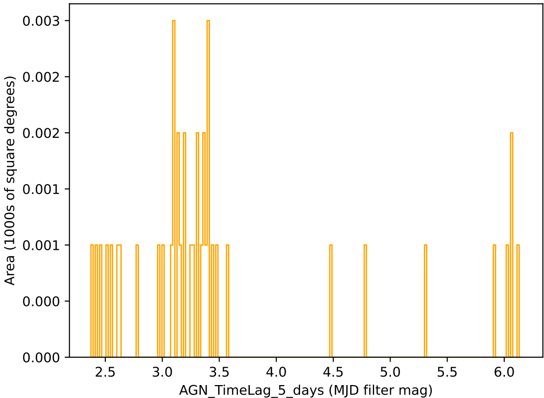
too_elab_r16_d2_gz_v3.4_10yrs r band: AGN_TimeLag_5_days
