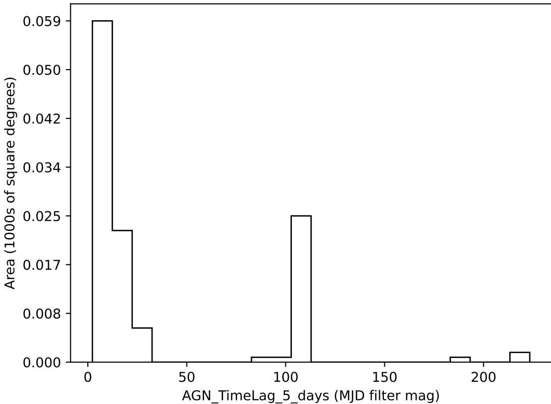
too_elab_r16_d2_gz_v3.4_10yrs all bands: AGN_TimeLag_5_days
