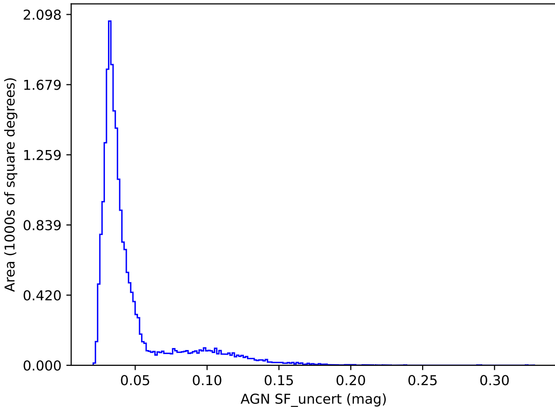
too_elab_r16_d2_gz_v3.4_10yrs y band: AGN SF_uncert
