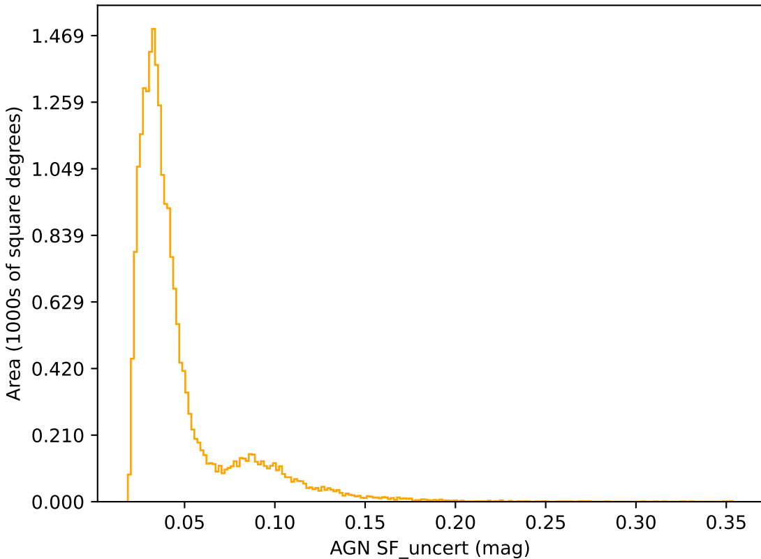
too_elab_r16_d2_gz_v3.4_10yrs r band: AGN SF_uncert
