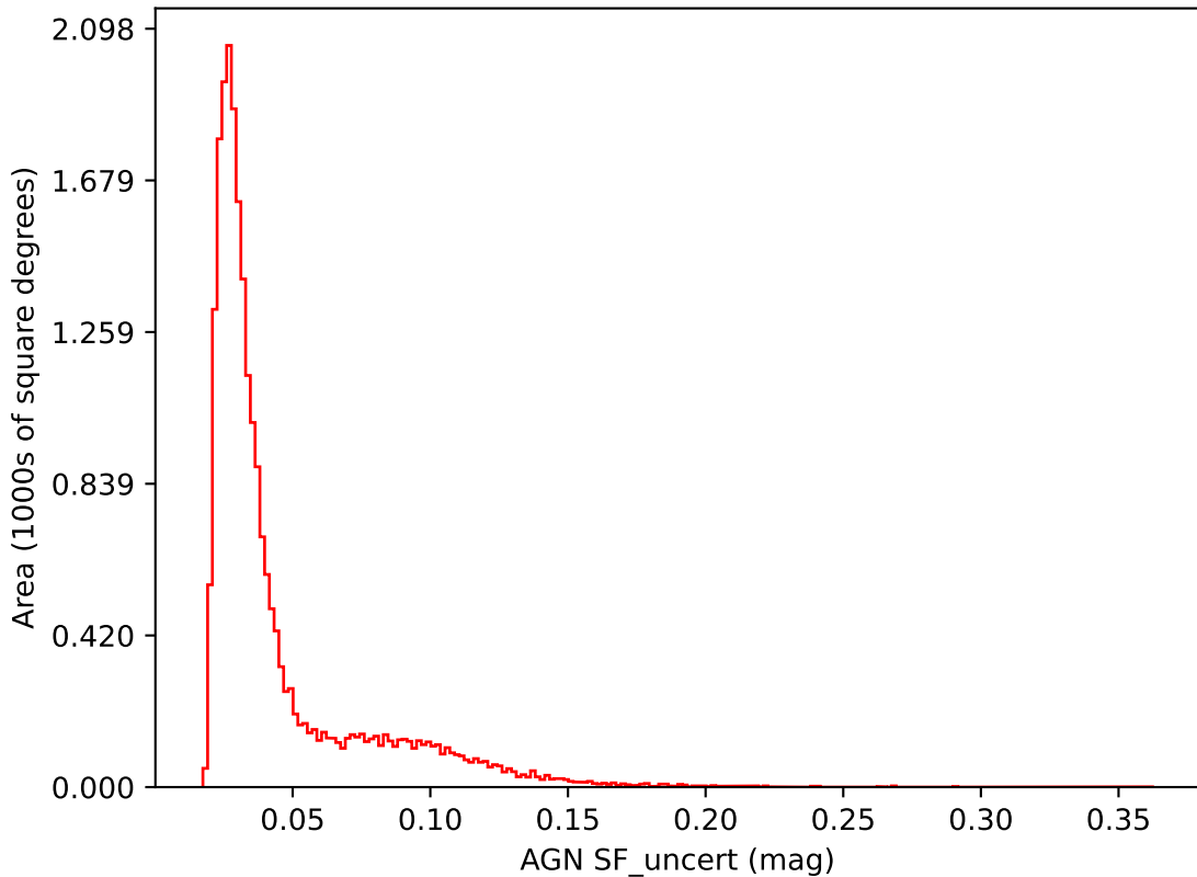
too_elab_r16_d2_gz_v3.4_10yrs i band: AGN SF_uncert
