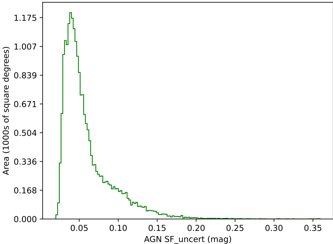
too_elab_r16_d2_gz_v3.4_10yrs g band: AGN SF_uncert
