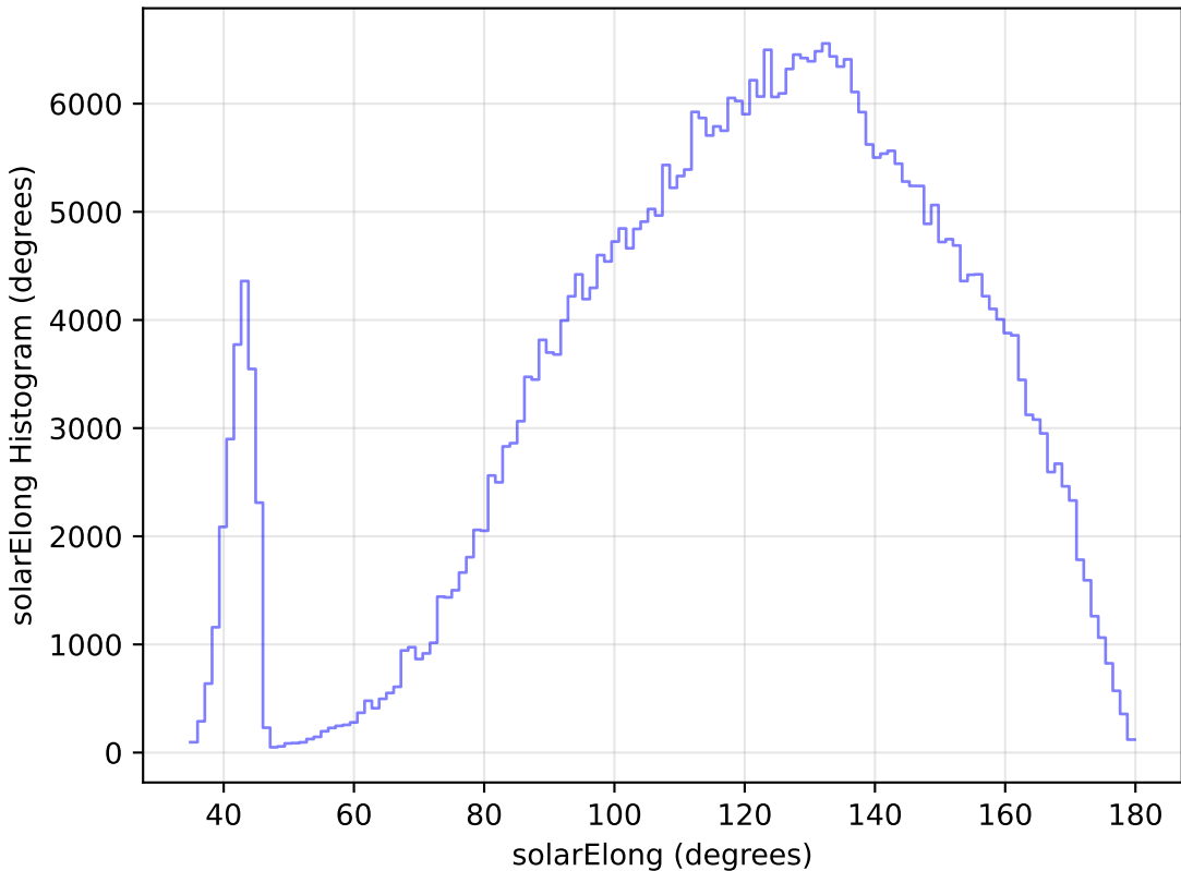
too_elab_r16_d2_gz_v3.4_10yrs WFD z band: solarElong Histogram
