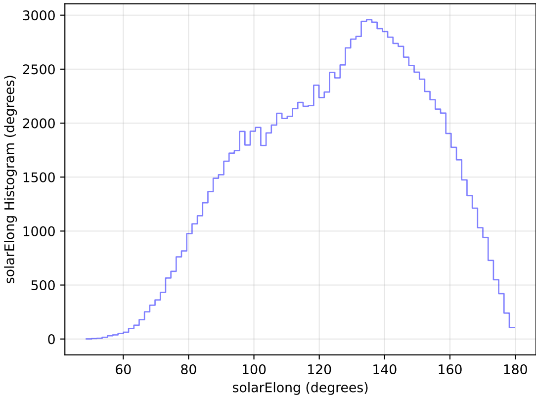
too_elab_r16_d2_gz_v3.4_10yrs WFD u band: solarElong Histogram
