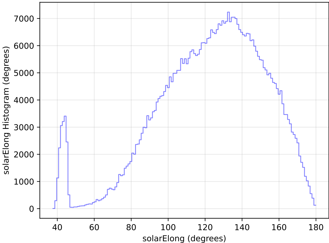
too_elab_r16_d2_gz_v3.4_10yrs WFD r band: solarElong Histogram
