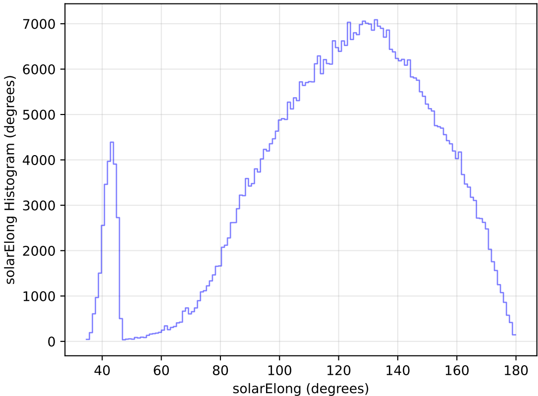
too_elab_r16_d2_gz_v3.4_10yrs WFD i band: solarElong Histogram
