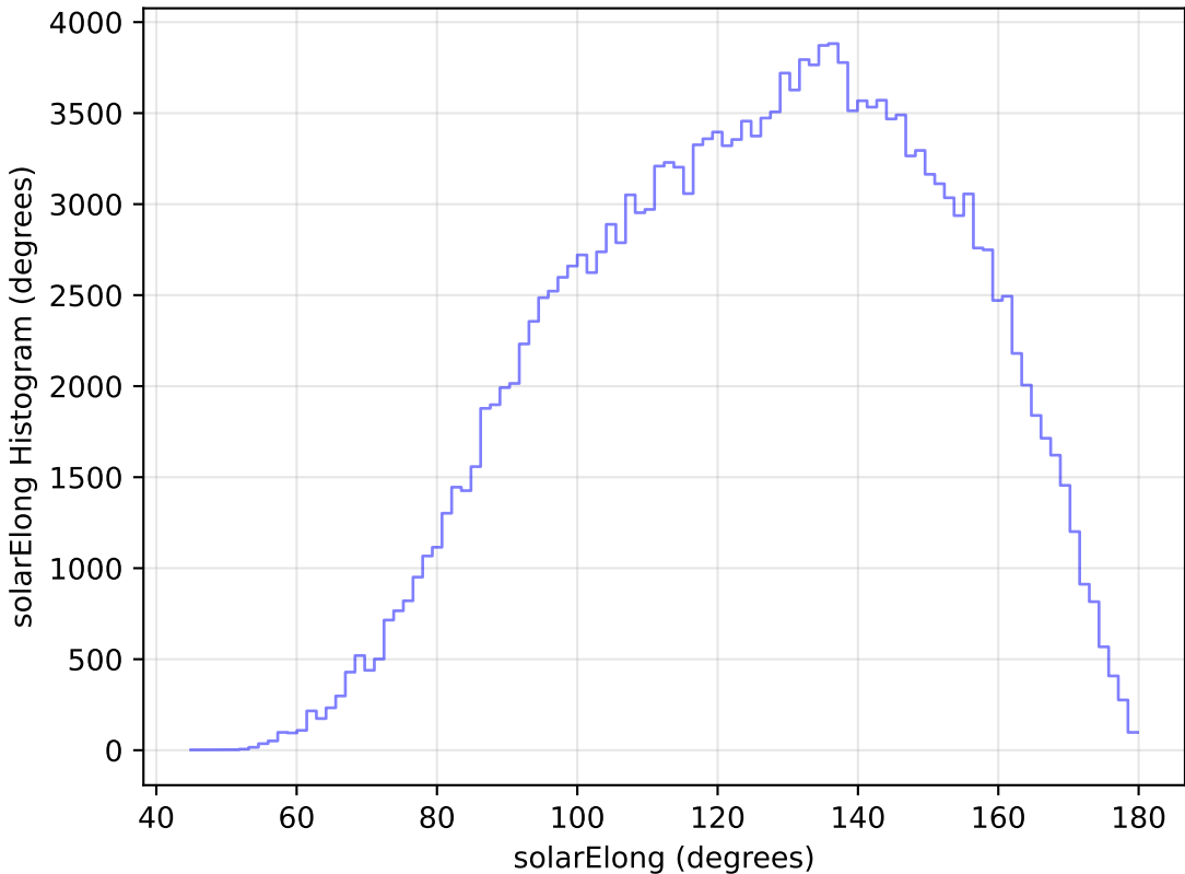
too_elab_r16_d2_gz_v3.4_10yrs WFD g band: solarElong Histogram
