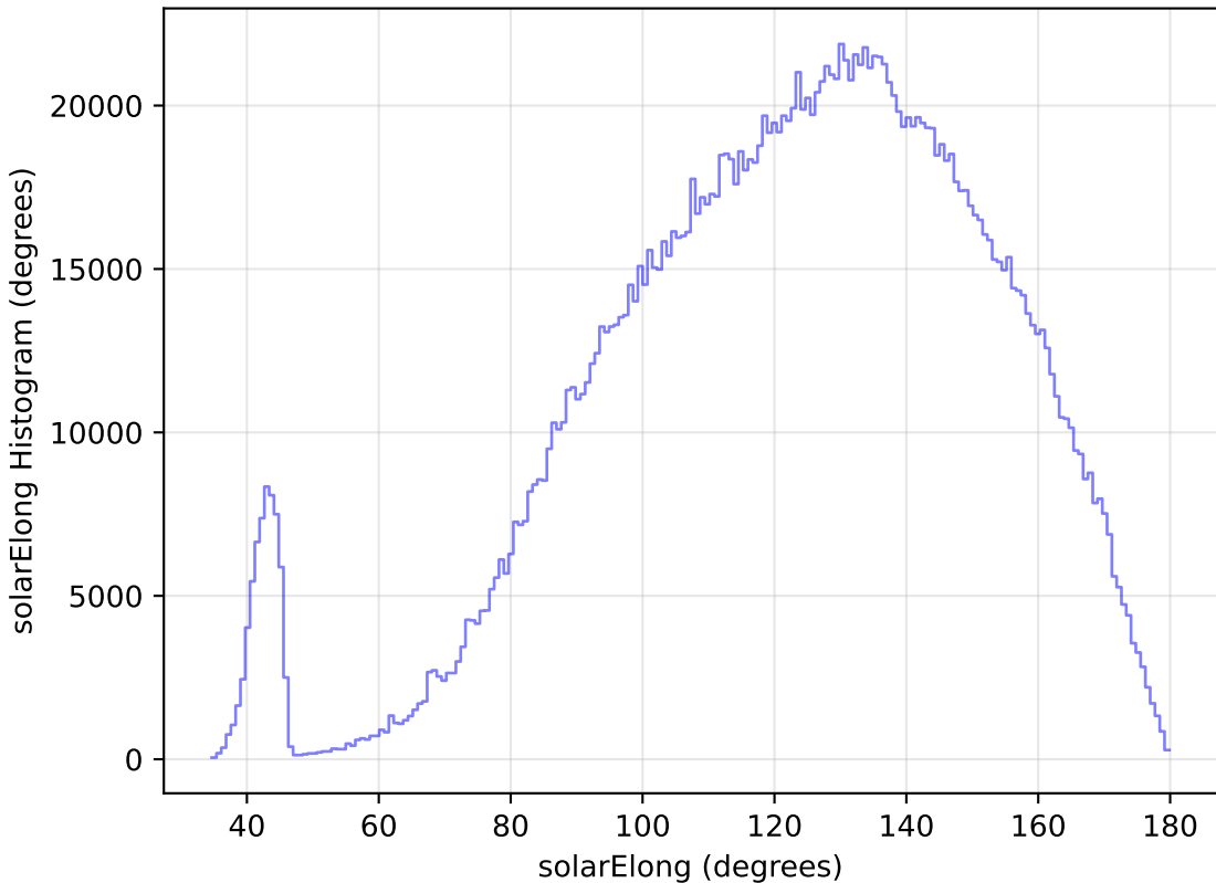
too_elab_r16_d2_gz_v3.4_10yrs WFD all bands: solarElong Histogram
