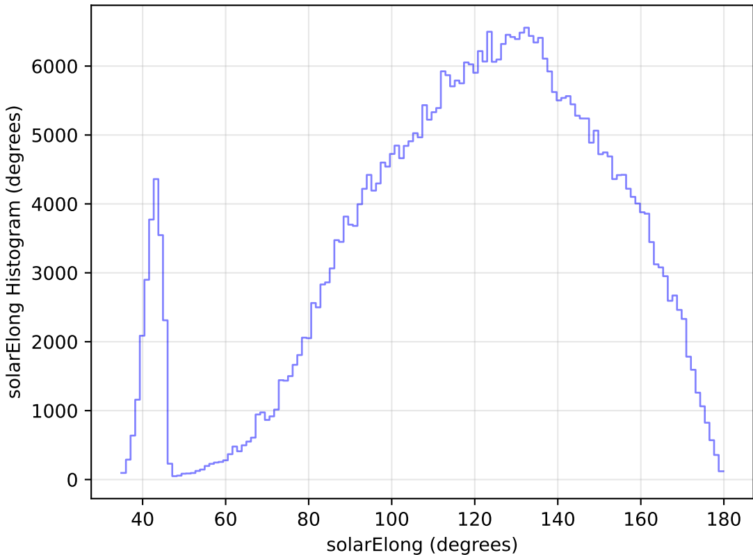
too_elab_r16_d2_gz_v3.4_10yrs All sky z band: solarElong Histogram
