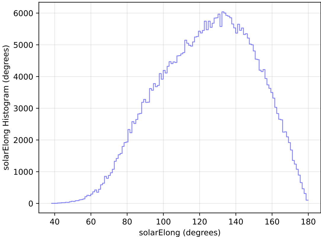
too_elab_r16_d2_gz_v3.4_10yrs All sky y band: solarElong Histogram
