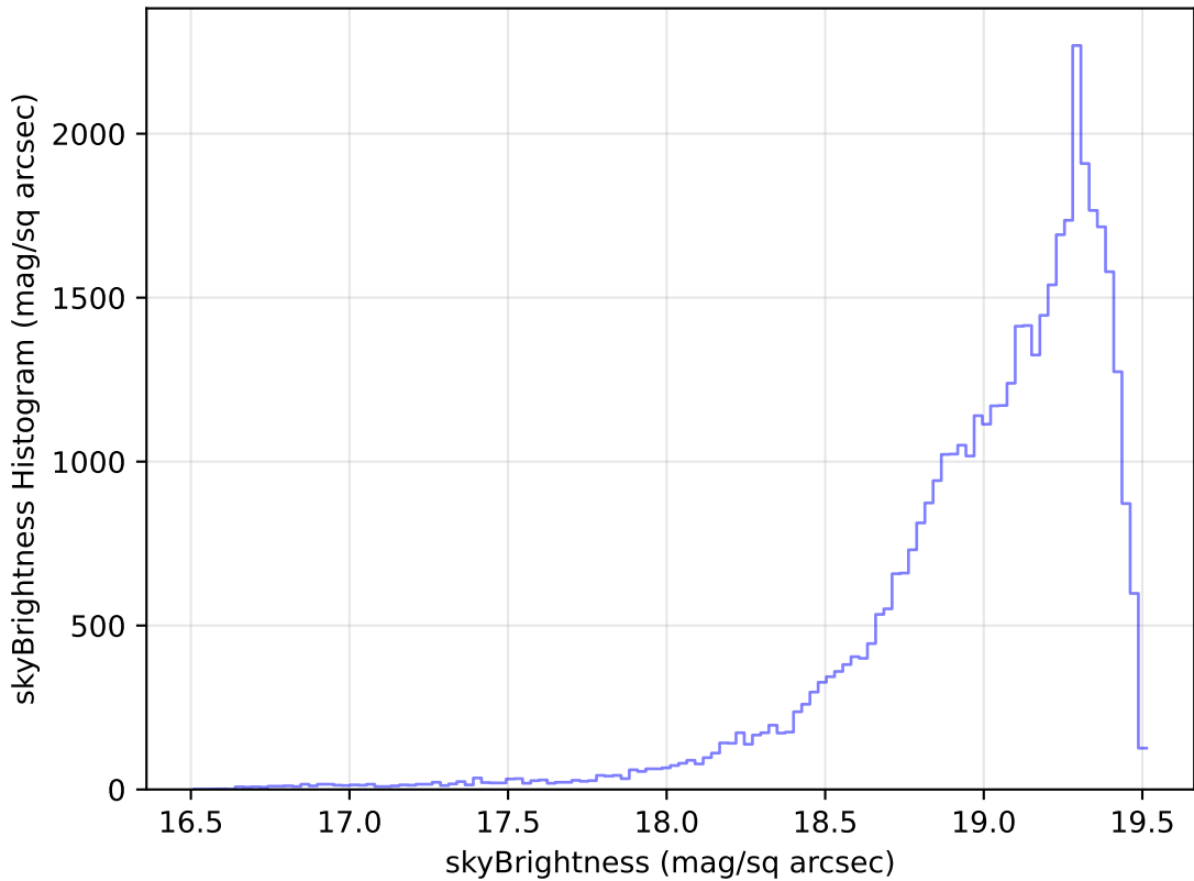
too_elab_r16_d2_gz_v3.4_10yrs Yr 1 z band: skyBrightness Histogram
