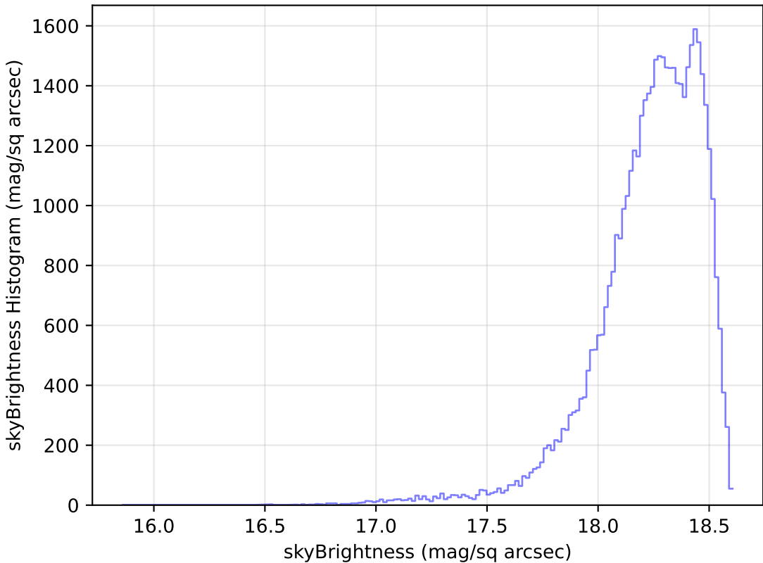
too_elab_r16_d2_gz_v3.4_10yrs Yr 1 y band: skyBrightness Histogram
