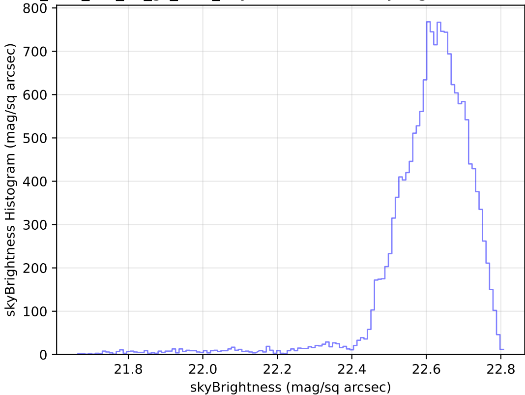
too_elab_r16_d2_gz_v3.4_10yrs Yr 1 u band: skyBrightness Histogram
