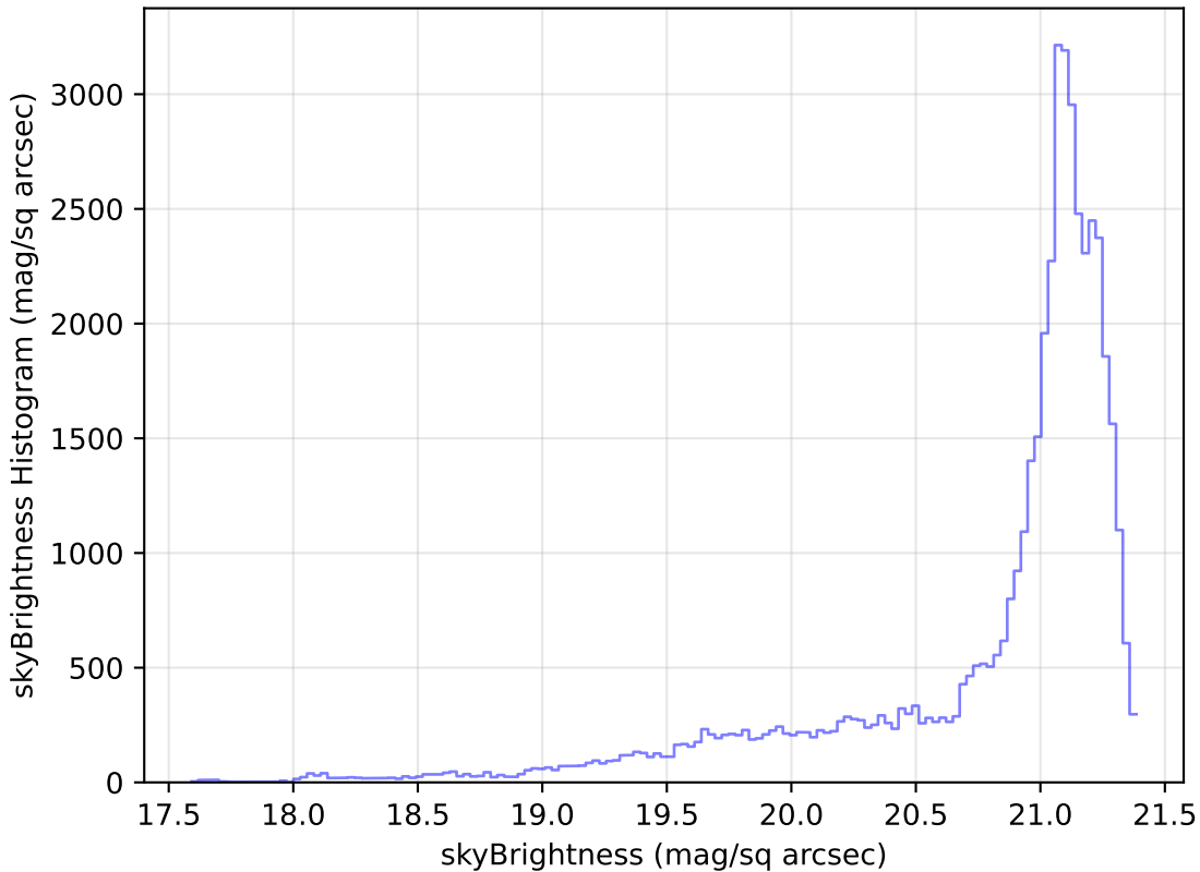
too_elab_r16_d2_gz_v3.4_10yrs Yr 1 r band: skyBrightness Histogram
