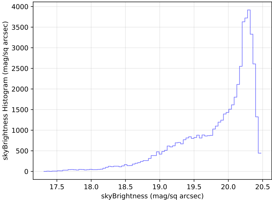
too_elab_r16_d2_gz_v3.4_10yrs Yr 1 i band: skyBrightness Histogram
