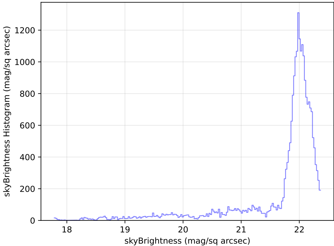
too_elab_r16_d2_gz_v3.4_10yrs Yr 1 g band: skyBrightness Histogram
