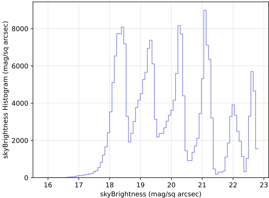
too_elab_r16_d2_gz_v3.4_10yrs Yr 1 all bands: skyBrightness Histogram
