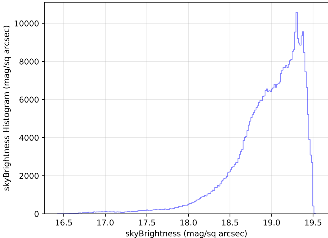
too_elab_r16_d2_gz_v3.4_10yrs WFD z band: skyBrightness Histogram
