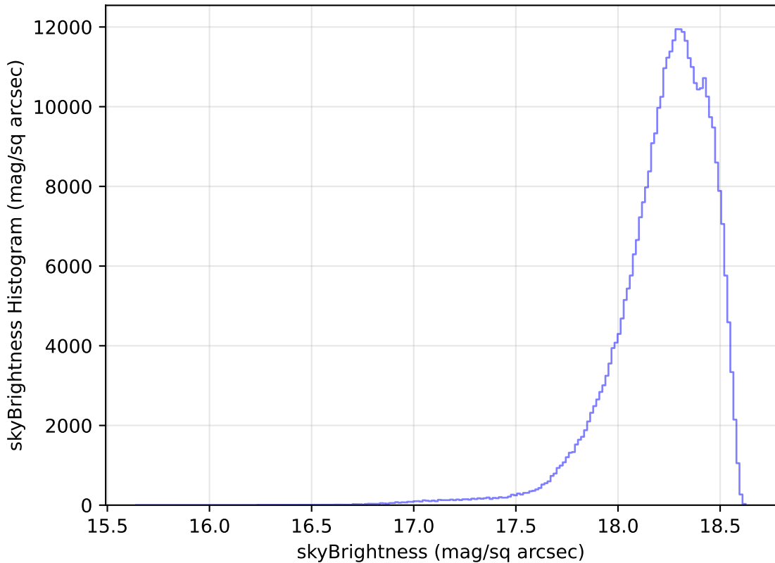
too_elab_r16_d2_gz_v3.4_10yrs WFD y band: skyBrightness Histogram
