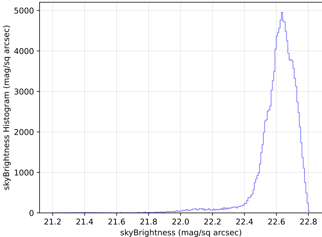
too_elab_r16_d2_gz_v3.4_10yrs WFD u band: skyBrightness Histogram
