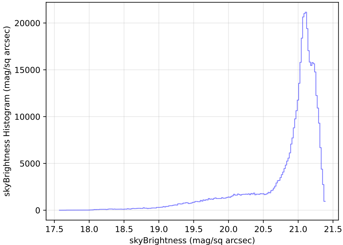
too_elab_r16_d2_gz_v3.4_10yrs WFD r band: skyBrightness Histogram
