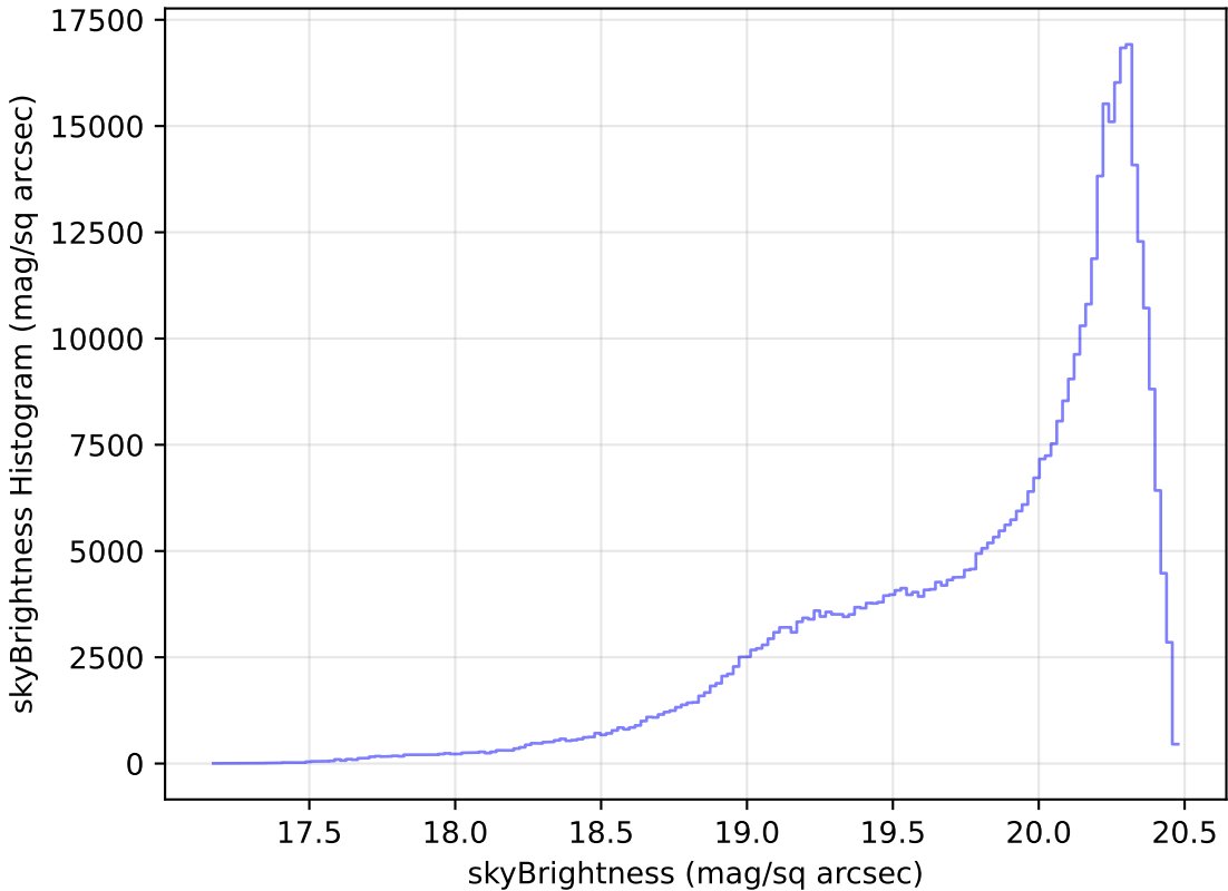
too_elab_r16_d2_gz_v3.4_10yrs WFD i band: skyBrightness Histogram
