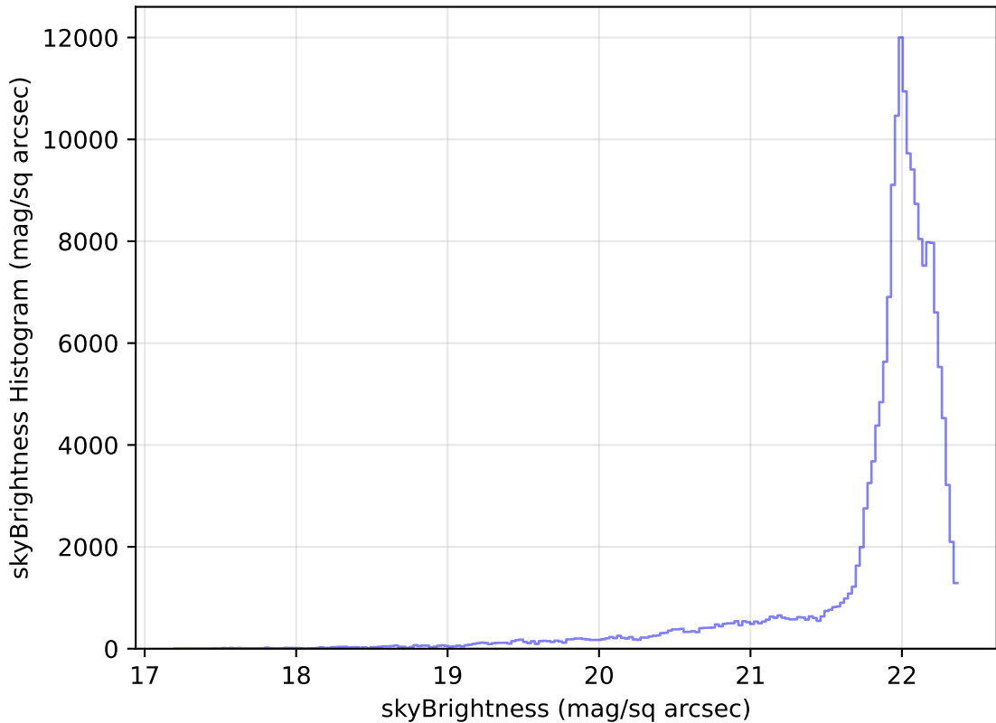
too_elab_r16_d2_gz_v3.4_10yrs WFD g band: skyBrightness Histogram
