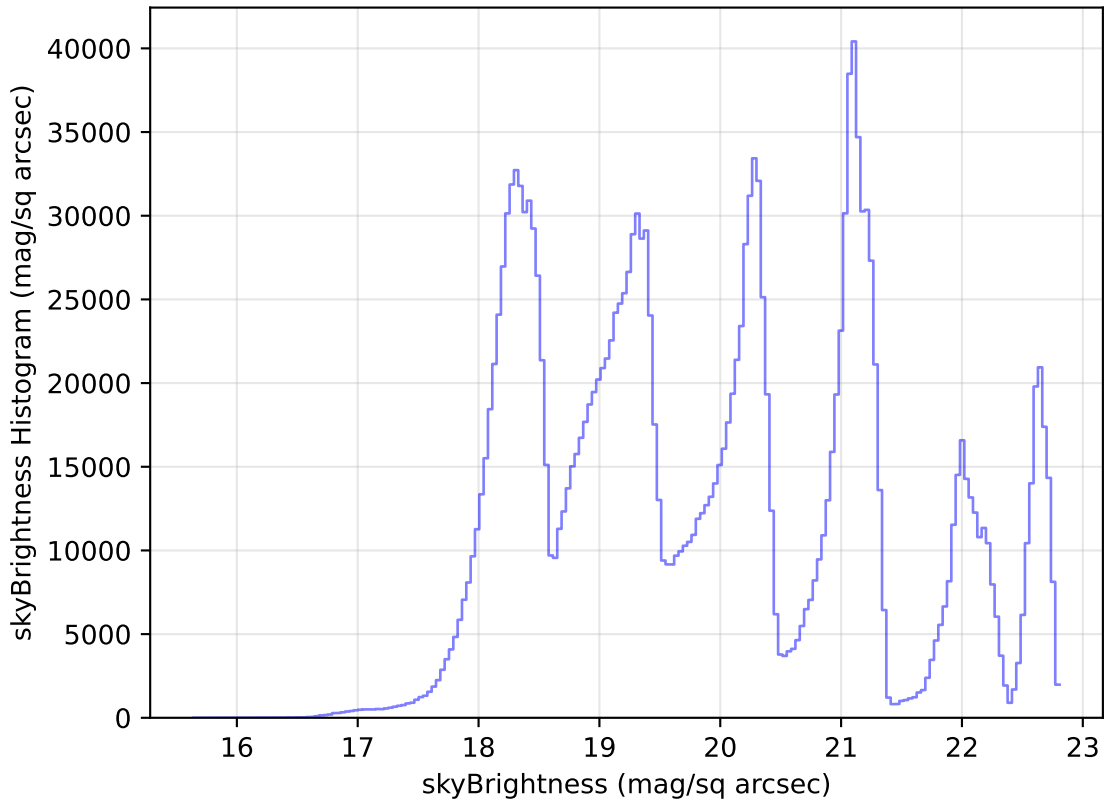
too_elab_r16_d2_gz_v3.4_10yrs WFD all bands: skyBrightness Histogram
