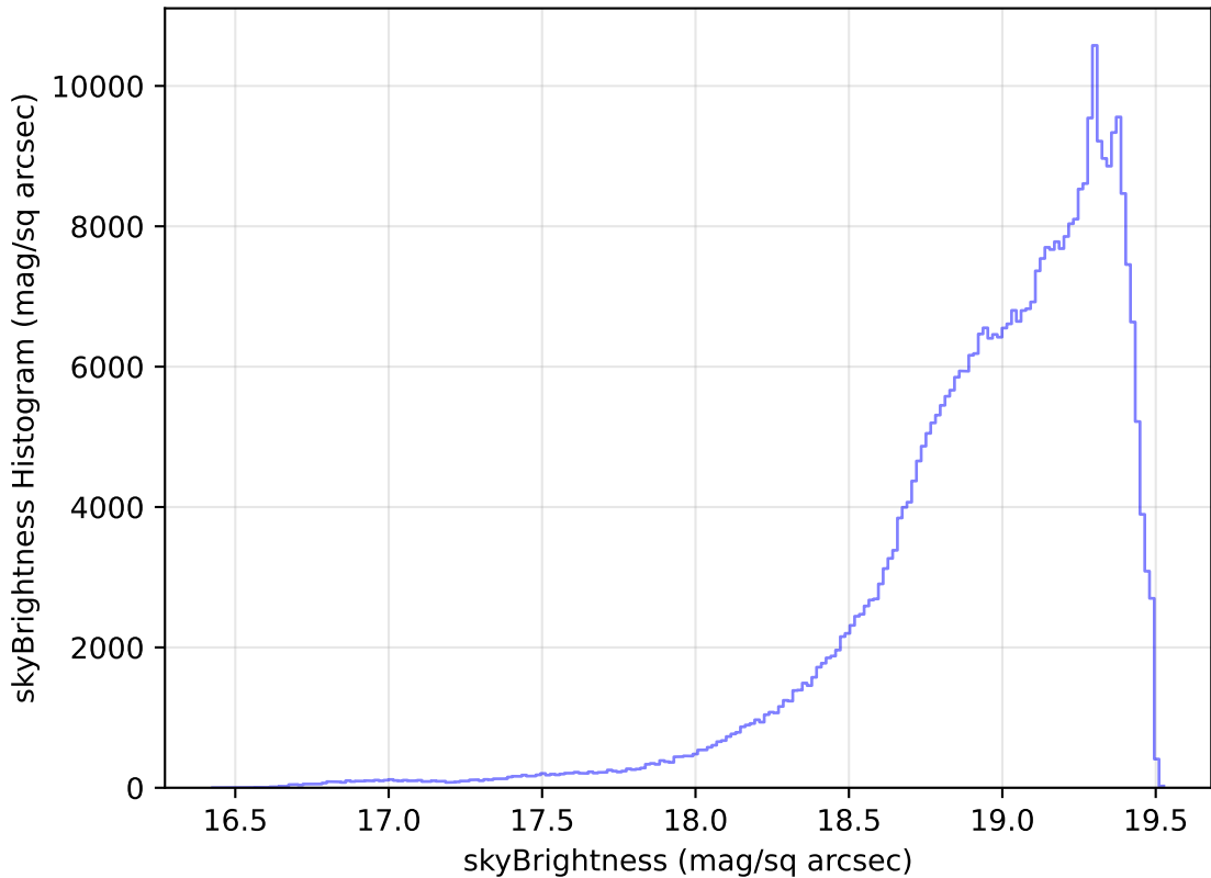
too_elab_r16_d2_gz_v3.4_10yrs All sky z band: skyBrightness Histogram
