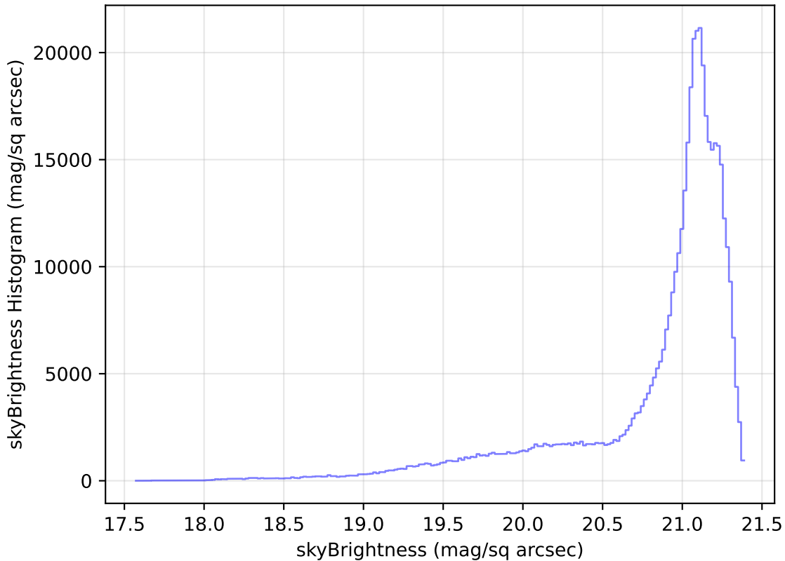
too_elab_r16_d2_gz_v3.4_10yrs All sky r band: skyBrightness Histogram
