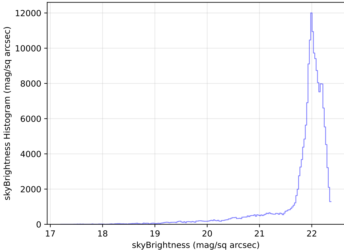
too_elab_r16_d2_gz_v3.4_10yrs All sky g band: skyBrightness Histogram
