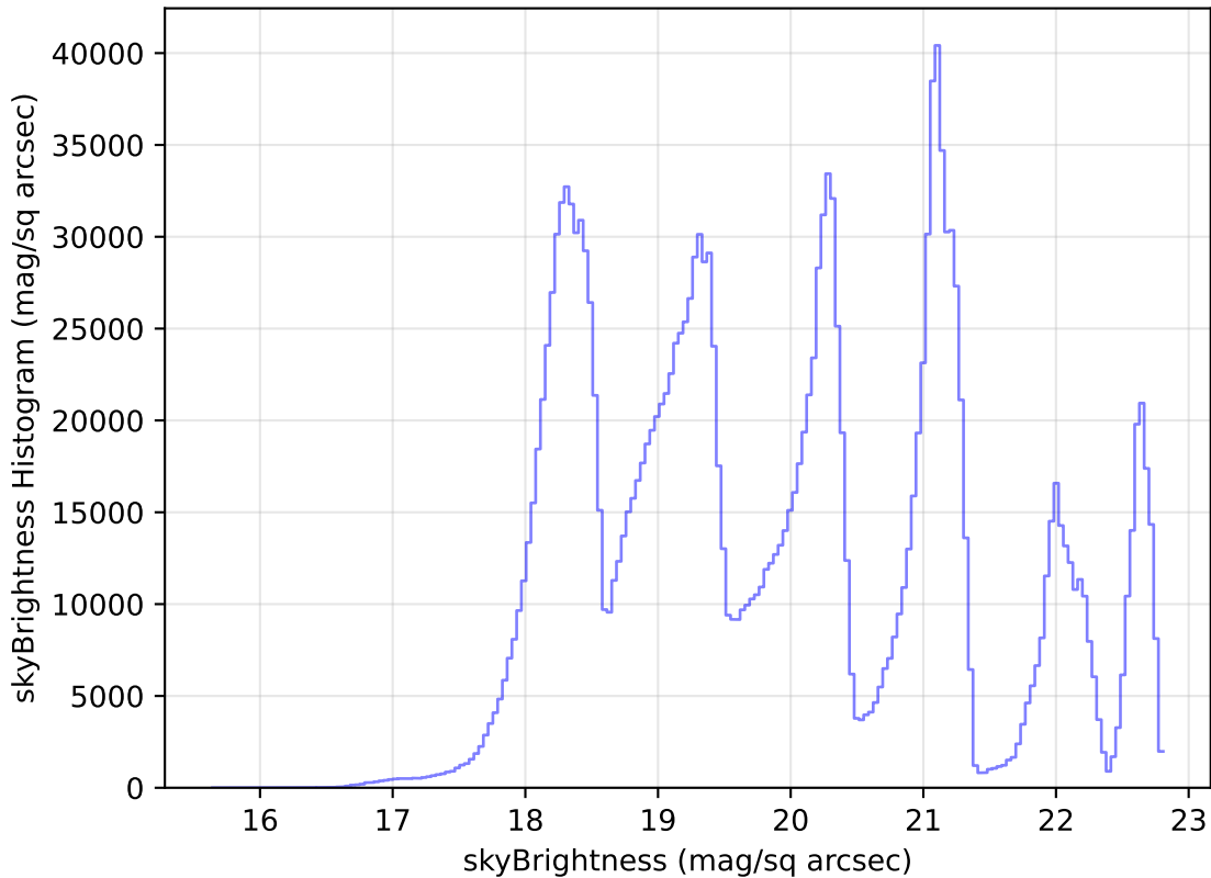
too_elab_r16_d2_gz_v3.4_10yrs All sky all bands: skyBrightness Histogram
