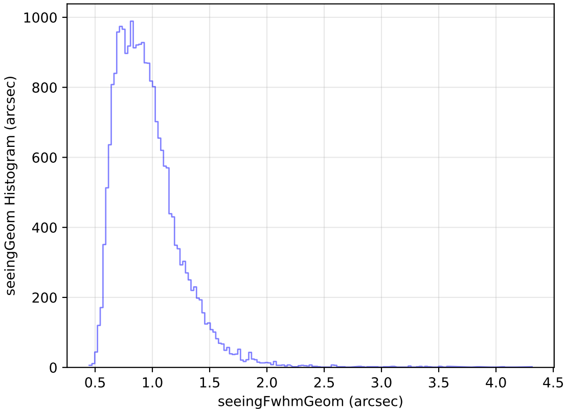
too_elab_r16_d2_gz_v3.4_10yrs Yr 1 g band: seeingGeom Histogram
