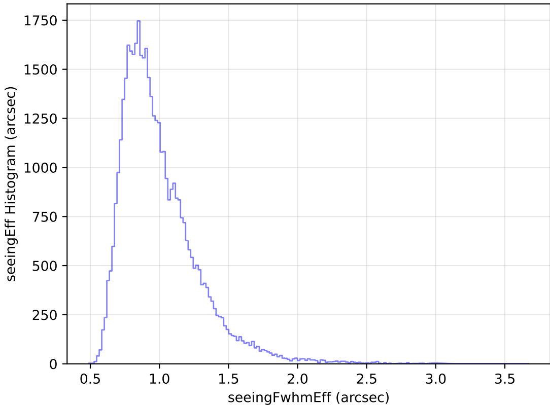
too_elab_r16_d2_gz_v3.4_10yrs Yr 1 z band: seeingEff Histogram
