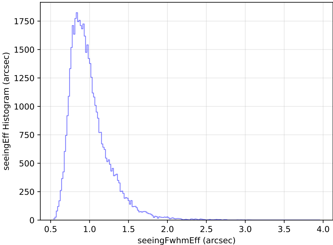
too_elab_r16_d2_gz_v3.4_10yrs Yr 1 y band: seeingEff Histogram
