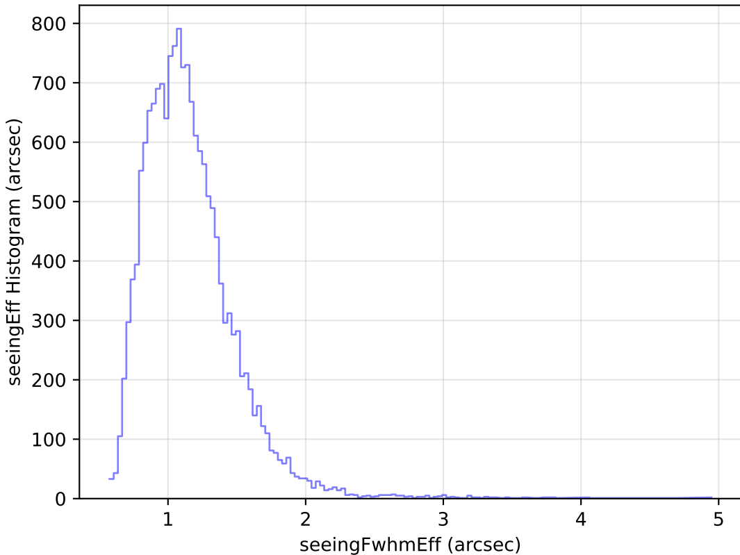
too_elab_r16_d2_gz_v3.4_10yrs Yr 1 u band: seeingEff Histogram
