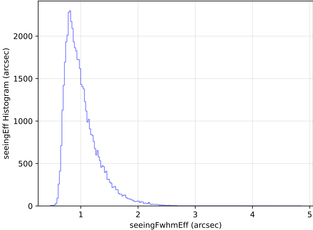
too_elab_r16_d2_gz_v3.4_10yrs Yr 1 r band: seeingEff Histogram
