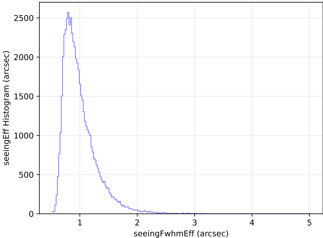
too_elab_r16_d2_gz_v3.4_10yrs Yr 1 i band: seeingEff Histogram
