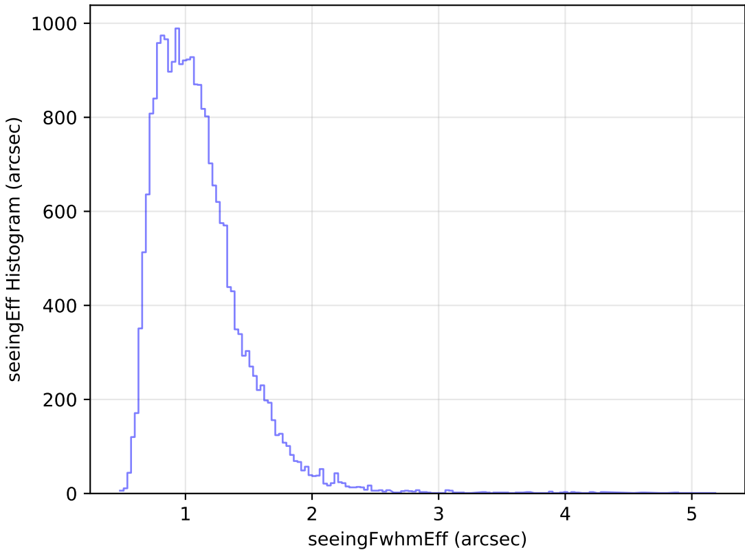
too_elab_r16_d2_gz_v3.4_10yrs Yr 1 g band: seeingEff Histogram
