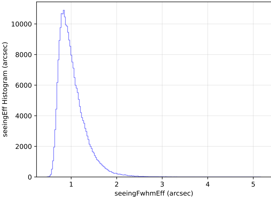
too_elab_r16_d2_gz_v3.4_10yrs Yr 1 all bands: seeingEff Histogram
