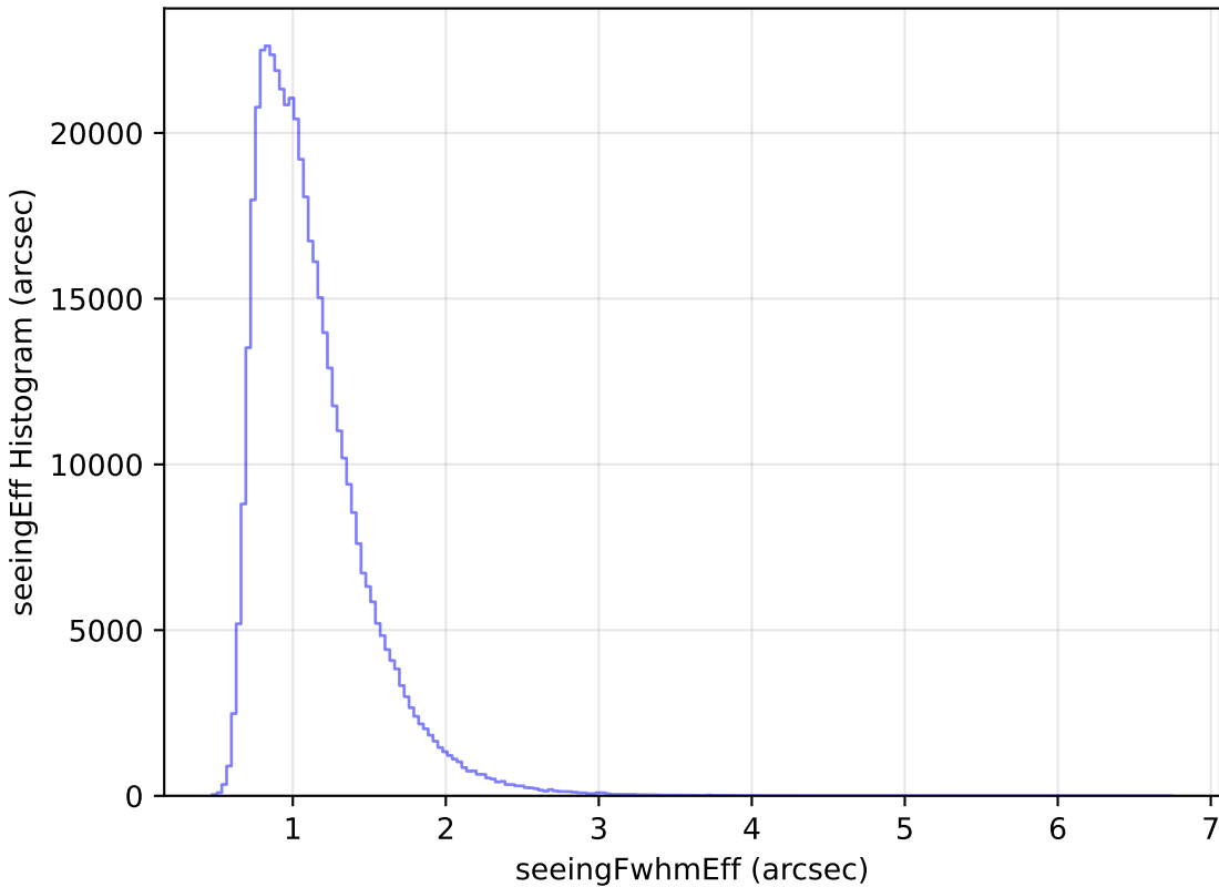
too_elab_r16_d2_gz_v3.4_10yrs WFD r band: seeingEff Histogram
