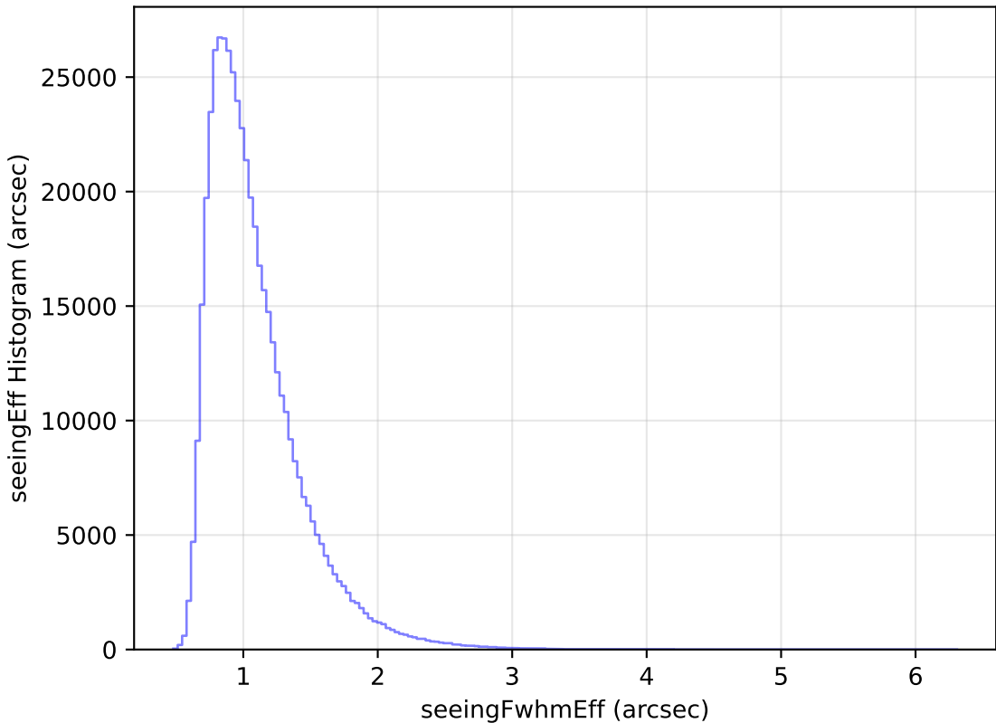
too_elab_r16_d2_gz_v3.4_10yrs WFD i band: seeingEff Histogram
