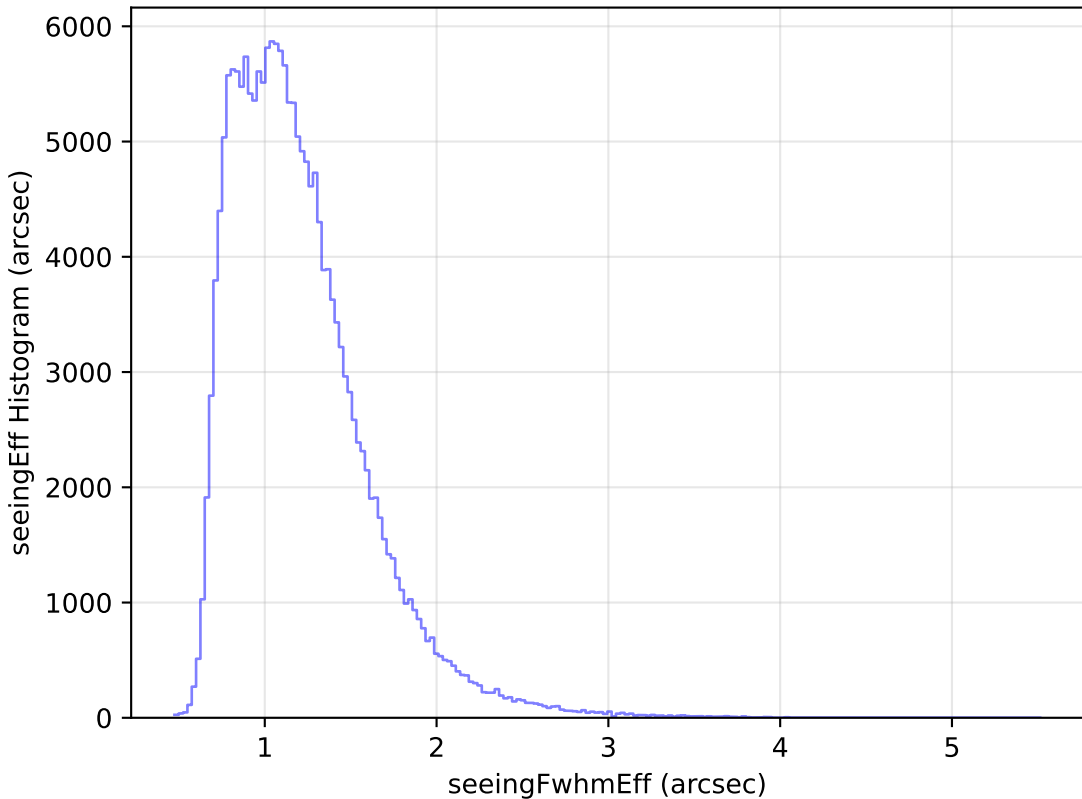
too_elab_r16_d2_gz_v3.4_10yrs WFD g band: seeingEff Histogram
