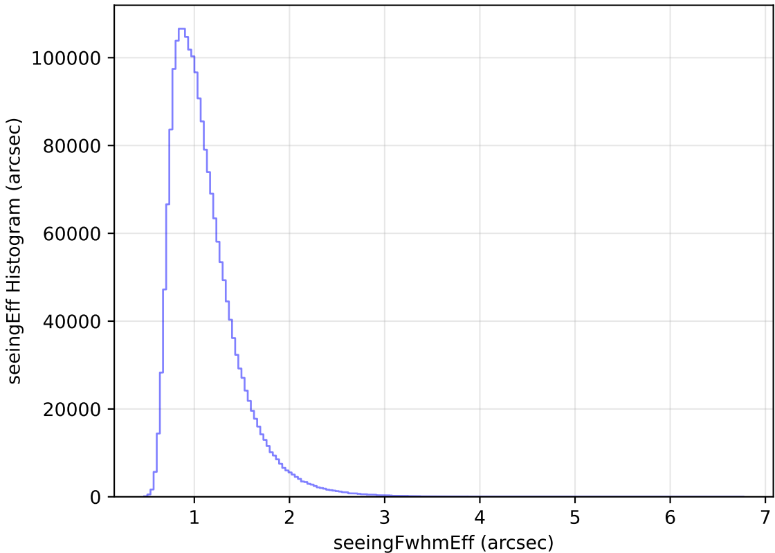
too_elab_r16_d2_gz_v3.4_10yrs WFD all bands: seeingEff Histogram
