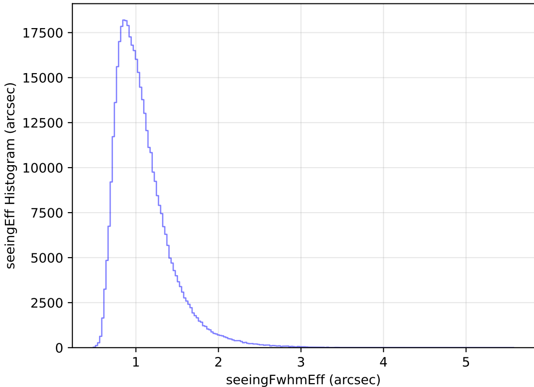
too_elab_r16_d2_gz_v3.4_10yrs All sky z band: seeingEff Histogram
