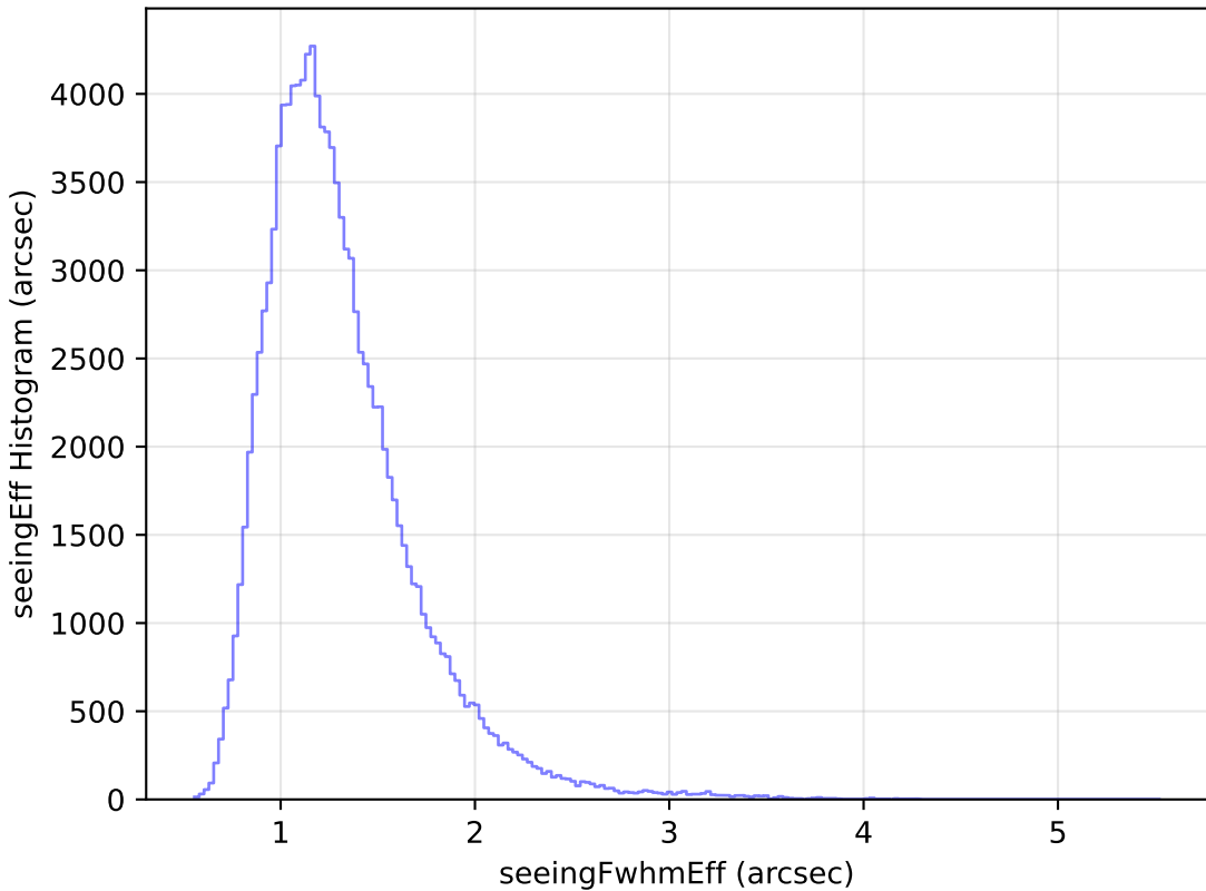
too_elab_r16_d2_gz_v3.4_10yrs All sky u band: seeingEff Histogram
