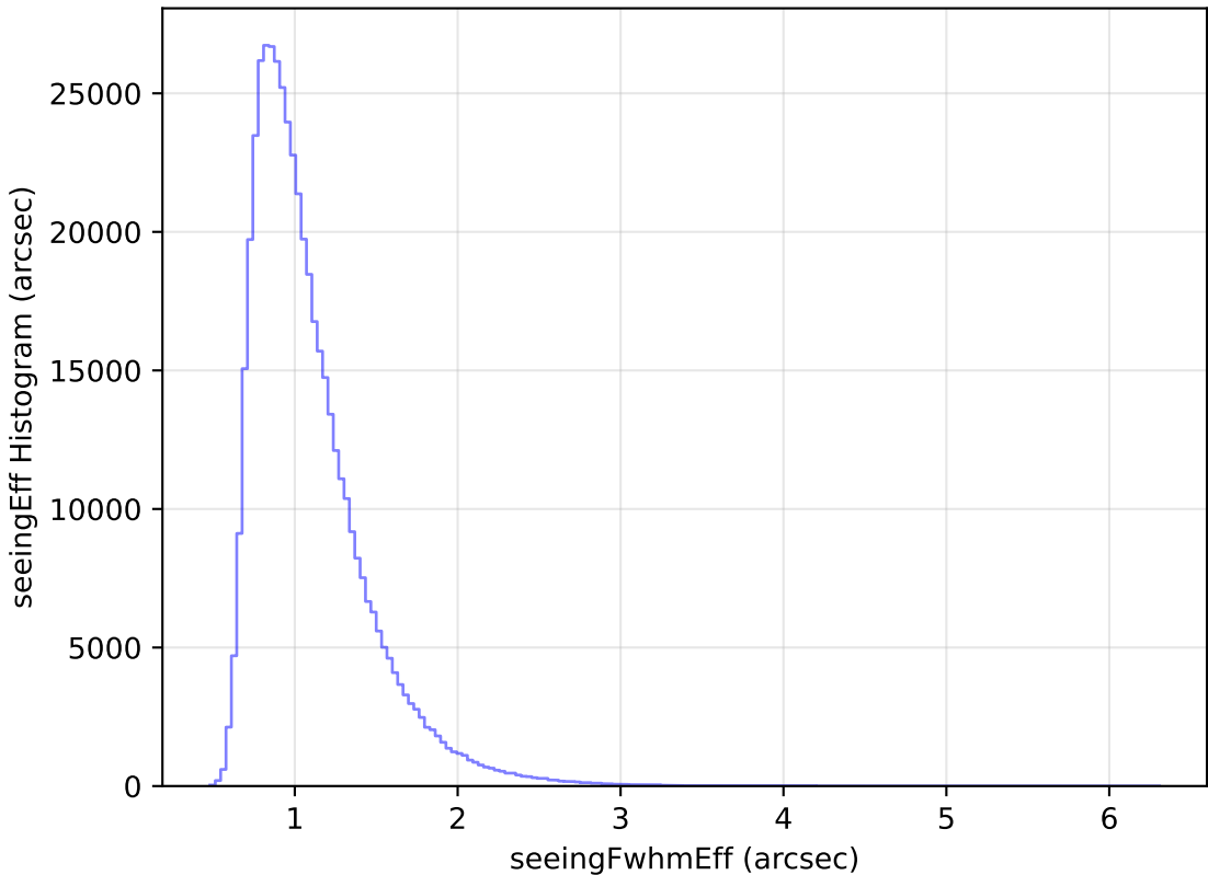
too_elab_r16_d2_gz_v3.4_10yrs All sky i band: seeingEff Histogram
