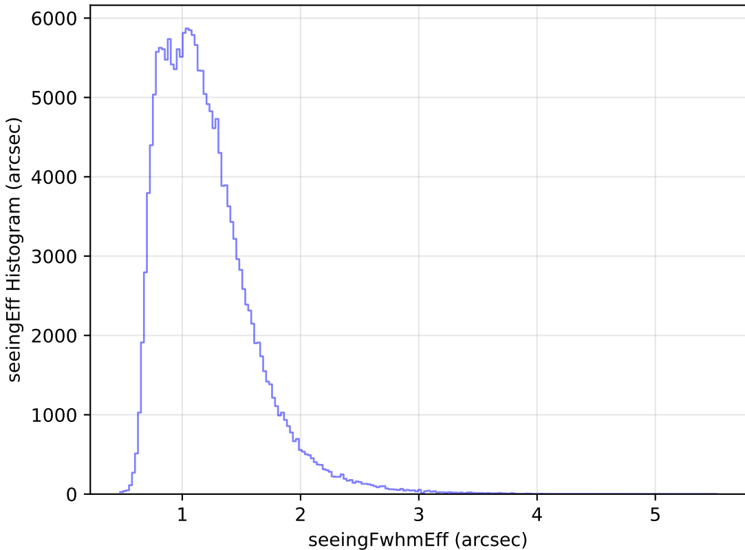
too_elab_r16_d2_gz_v3.4_10yrs All sky g band: seeingEff Histogram
