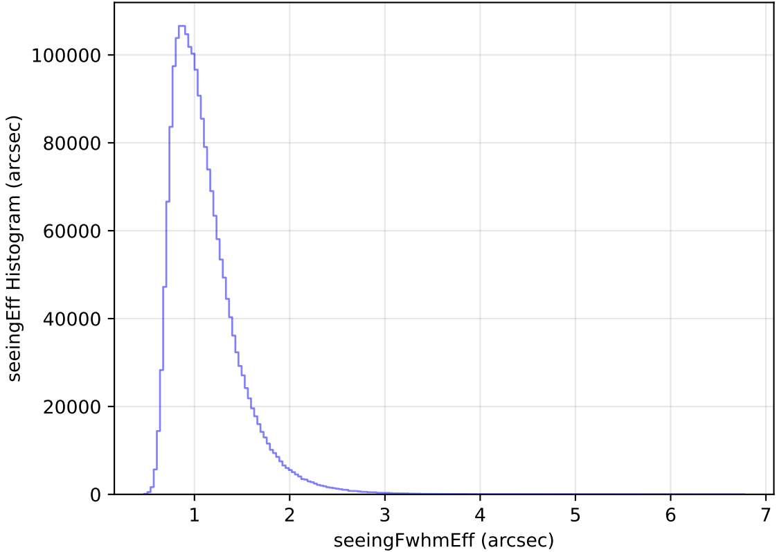
too_elab_r16_d2_gz_v3.4_10yrs All sky all bands: seeingEff Histogram
