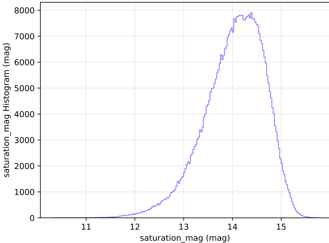
too_elab_r16_d2_gz_v3.4_10yrs WFD z band: saturation_mag Histogram
